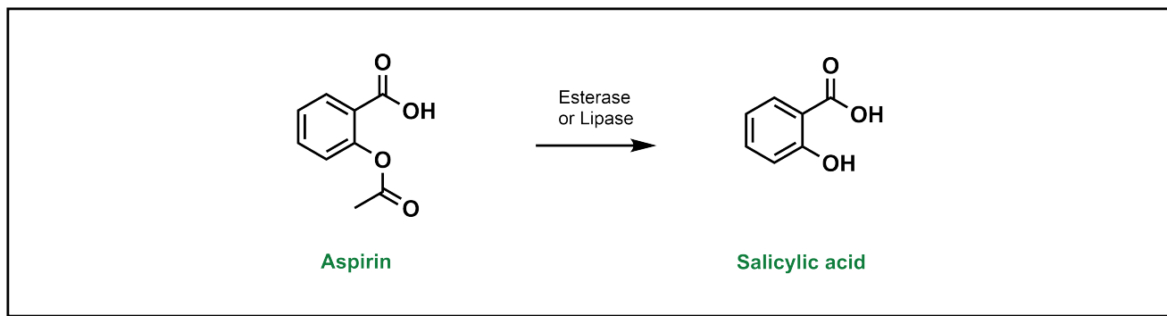
FIGURE 5.20 Aspirin can be hydrolyzed to salicylic acid.
