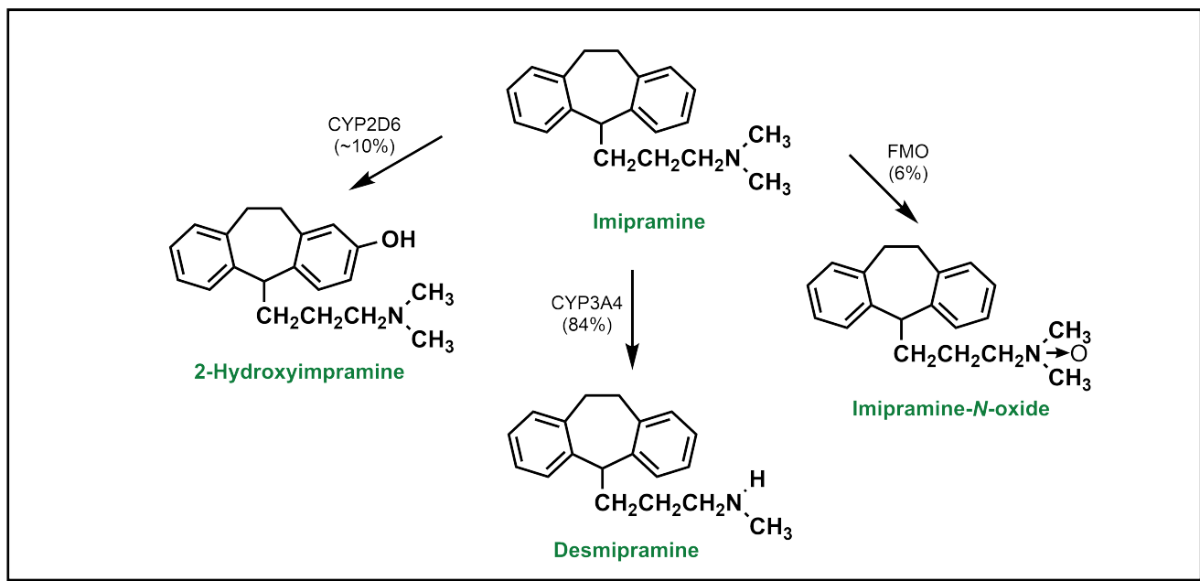
FIGURE 5.14 Oxidation route of imipramine. Desmipramine can be further metabolized by additional N-dealkylation or hydroxylation on the sp^3 ring system.
