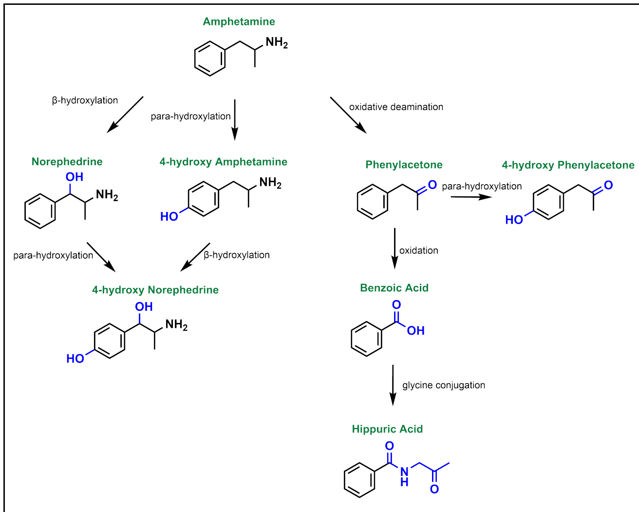
FIGURE 5.13 Differential metabolism routes of amphetamine.
