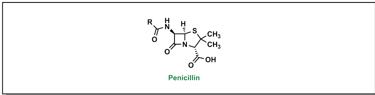
FIGURE 2.4 Structure of penicillin.
