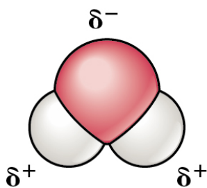
(b) Three-dimensional model of a water molecule
