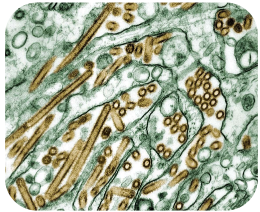
Figure 4.1.4 This transmission electron micrograph shows the inside of cells where you can see it is invaded with viruses (in brown). Image by Cynthia Goldsmith, USCD CP, CC0 1.0
