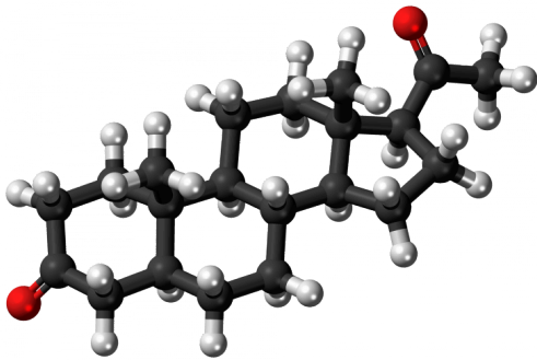
Figure 3.3.7 Progesterone is an example of a steroid. Image by Jynto, CC0 BY 1.0
