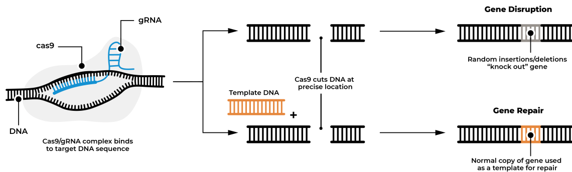
Figure 10.1.9 CRISPR gRNA binds at a target DNA sequence then Cas9 cuts the DNA. This can be done to “knock out” a gene or to use a DNA template to repair a gene. Image modification of work by Ianis G. Matsoukas, CC BY 4.0 Mods: terminology updated, labels clarified, layout refined.
