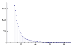
Power Law Distribution CC BY SA image from Giuseppe Vitucci
