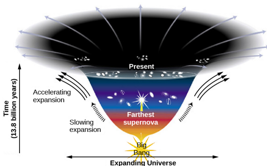
Figure 29.4. Changes in the Rate of Expansion of the Universe Since Its Beginning 13.8 Billion Years Ago. The more the diagram spreads out horizontally, the faster the change in the velocity of expansion. After a period of very rapid expansion at the beginning, which scientists call inflation and which we will discuss later in this chapter, the expansion began to decelerate. Galaxies were then close together, and their mutual gravitational attraction slowed the expansion. After a few billion years, when galaxies were farther apart, the influence of gravity began to weaken. Dark energy then took over and caused the expansion to accelerate. (credit: modification of work by Ann Feild (STScI))
