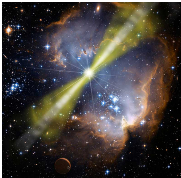
Figure 23.22. Burst That Is Beamed. This artist's conception shows an illustration of one kind of gamma-ray burst. The collapse of the core of a massive star into a black hole has produced two bright beams of light originating from the star's poles, which an observer pointed along one of these axes would see as a gamma-ray burst. The hot blue stars and gas clouds in the vicinity are meant to show that the event happened in an active star-forming region. (credit: NASA/Swift/Mary Pat Hrybyk-Keith and John Jones)
