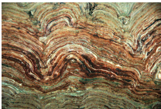
Figure 8.15. Cross-Sections of Fossil Stromatolites. This polished cross-section of a fossilized colony of stromatolites dates to the Precambrian Era. The layered, domelike structures are mats of sediment trapped in shallow waters by large numbers of blue-green bacteria that can photosynthesize. Such colonies of microorganisms date back more than 3 billion years. (credit: James St. John)
