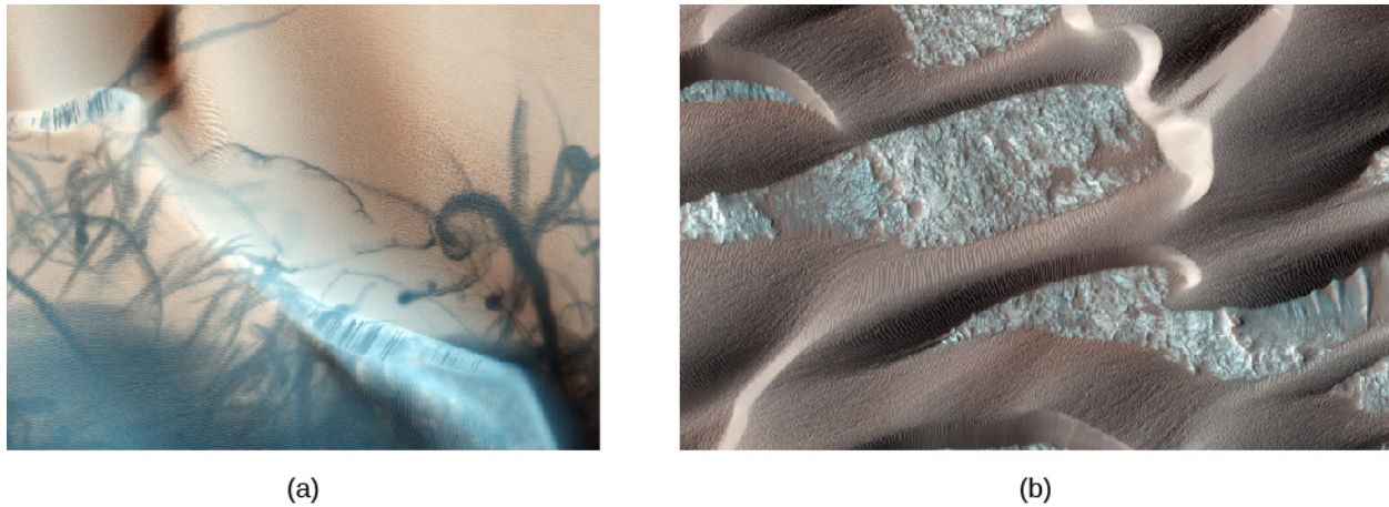
Figure 10.23. Dust Devil Tracks and Sand Dunes. (a) This high-resolution photo from the Mars Global Surveyor shows the dark tracks of several dust devils that have stripped away a thin coating of light-colored dust. This view is of an area about 3 kilometers across. Dust devils are one of the most important ways that dust gets redistributed by the martian winds. They may also help keep the solar panels of our rovers free of dust. (b) These windblown sand dunes on Mars overlay a lighter sandy surface. Each dune in this high-resolution view is about 1 kilometer across. (credit a: modification of work by NASA/JPL/University of Arizona; credit b: modification of work by NASA/JPL-Caltech/University of Arizona)
