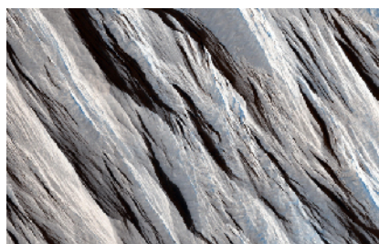
Figure 10.24. Wind Erosion on Mars. These long straight ridges, called yardangs, are aligned with the dominant wind direction. This is a high-resolution image from the Mars Reconnaissance Orbiter and is about 1 kilometer wide. (credit: NASA/JPL-Caltech/University of Arizona)
