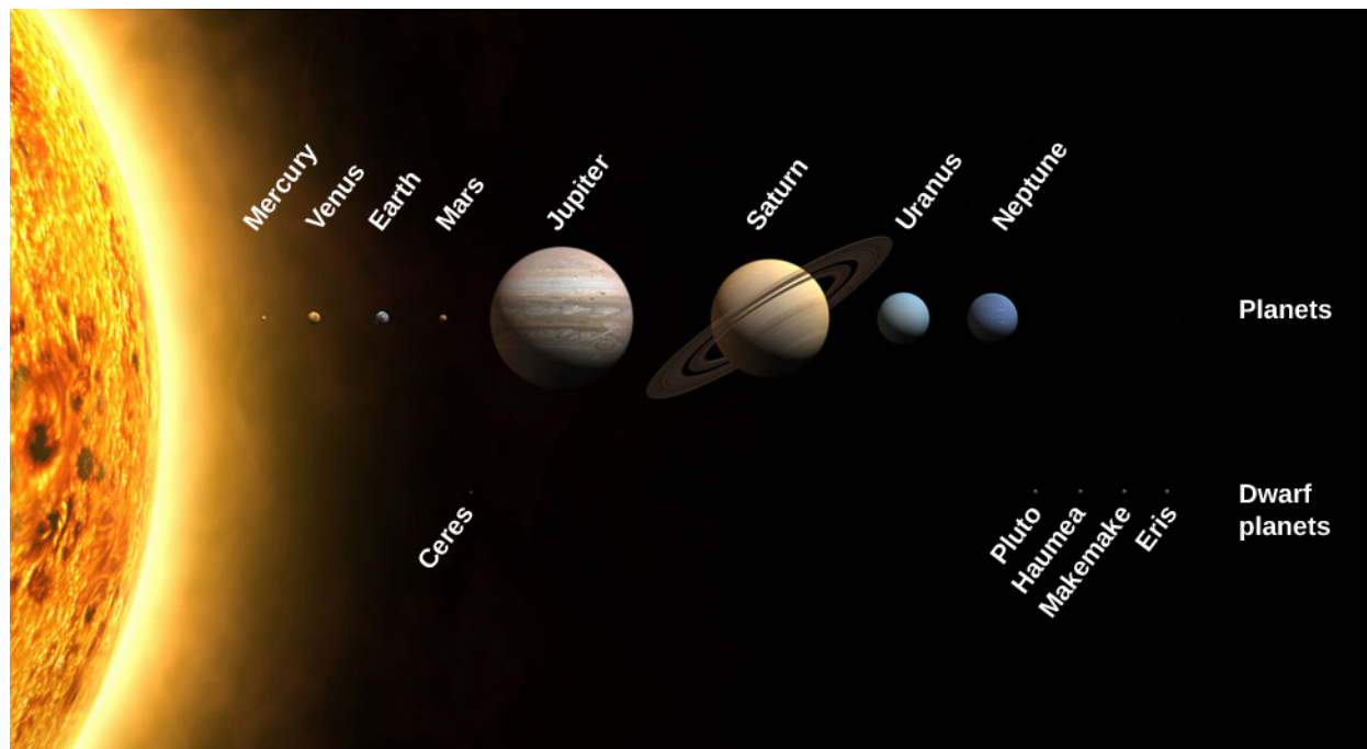
Figure 1.8. Our Solar Family. The Sun, the planets, and some dwarf planets are shown with their sizes drawn to scale. The orbits of the planets are much more widely separated than shown in this drawing. Notice the size of Earth compared to the giant planets. (credit: modification of work by NASA)
