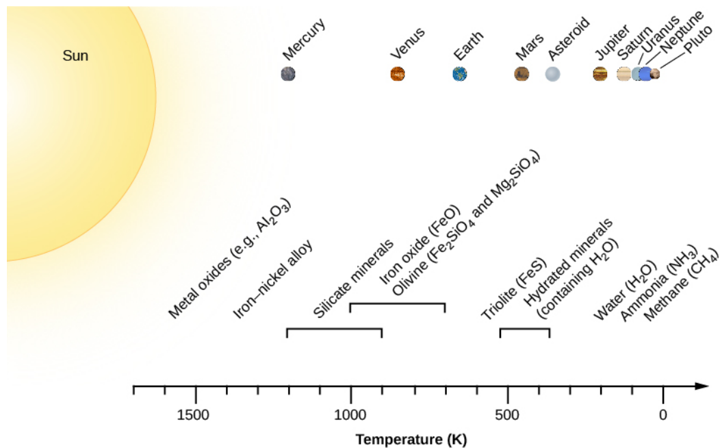
Figure 14.12. Chemical Condensation Sequence in the Solar Nebula. The scale along the bottom shows temperature; above are the materials that would condense out at each temperature under the conditions expected to prevail in the nebula.
