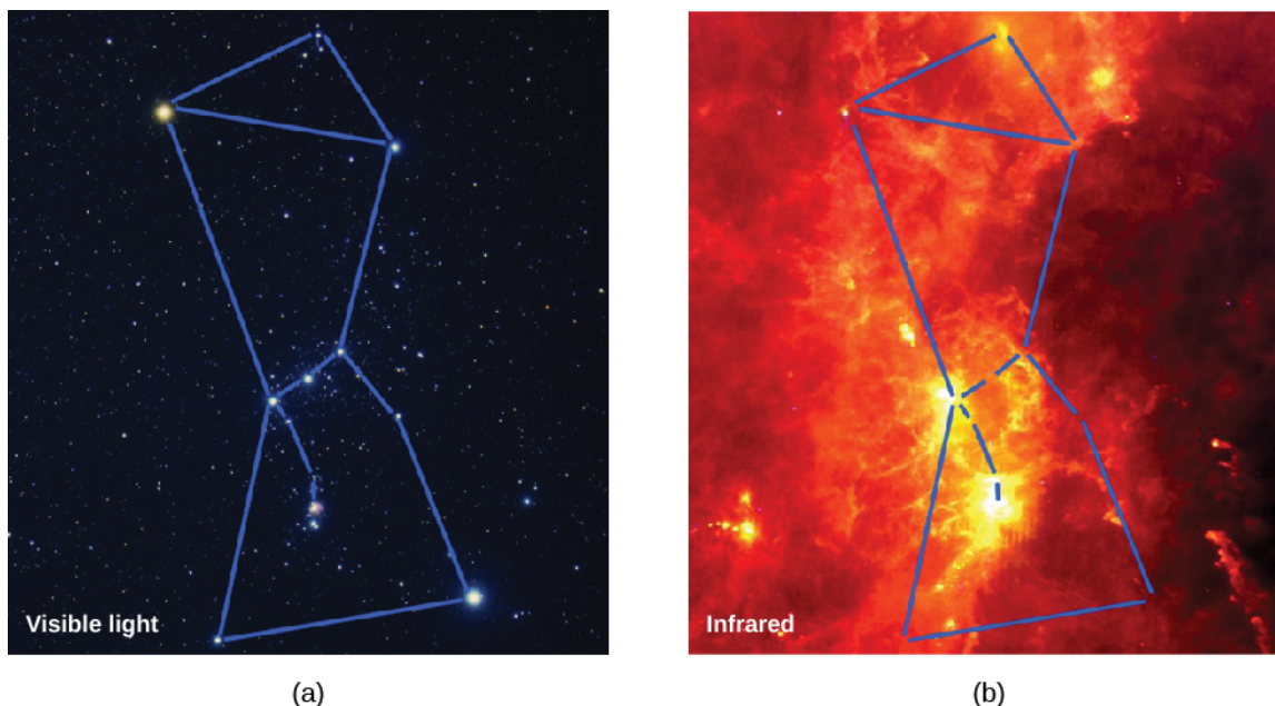
Figure 21.3. Orion in Visible and Infrared. (a) The Orion star group was named after the legendary hunter in Greek mythology. Three stars close together in a line mark Orion's belt. The ancients imagined a sword hanging from the belt; the object at the end of the blue line in this sword is the Orion Nebula. (b) This wide-angle, infrared view of the same area was taken with the Infrared Astronomical Satellite. Heated dust clouds dominate in this false-color image, and many of the stars that stood out on part (a) are now invisible. An exception is the cool, red-giant star Betelgeuse, which can be seen as a yellowish point at the left vertex of the blue triangle (at Orion's left armpit). The large, yellow ring to the right of Betelgeuse is the remnant of an exploded star. The infrared image lets us see how large and full of cooler material the Orion molecular cloud really is. On the visible-light image at left, you see only two colorful regions of interstellar matter—the two, bright yellow splotches at the left end of and below Orion's belt. The lower one is the Orion Nebula and the higher one is the region of the Horsehead Nebula. (credit: modification of work by NASA, visible light: Akira Fujii; infrared: Infrared Astronomical Satellite)
