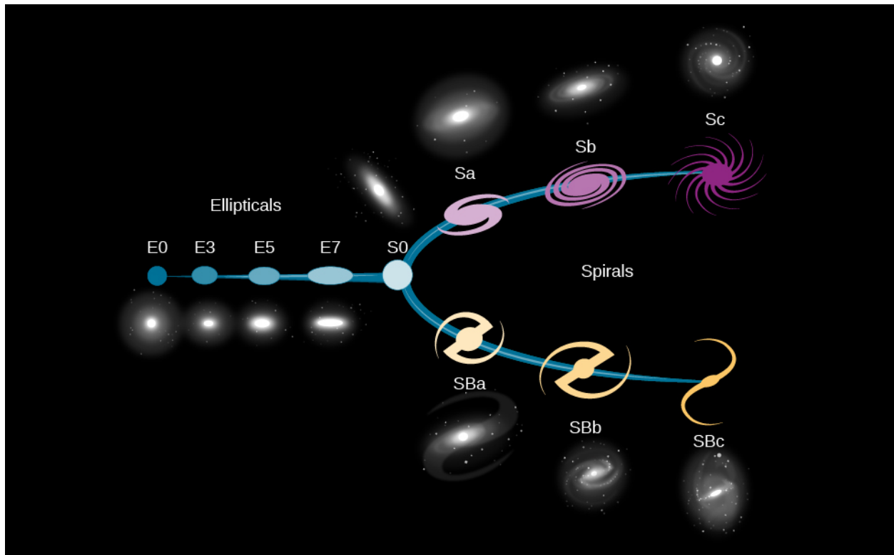
Figure 26.6. Hubble Classification of Galaxies. This figure shows Edwin Hubble's original classification of galaxies. Elliptical galaxies are on the left. On the right, you can see the basic spiral shapes illustrated, alongside images of actual barred and unbarred spirals. (credit: modification of work by NASA, ESA)
