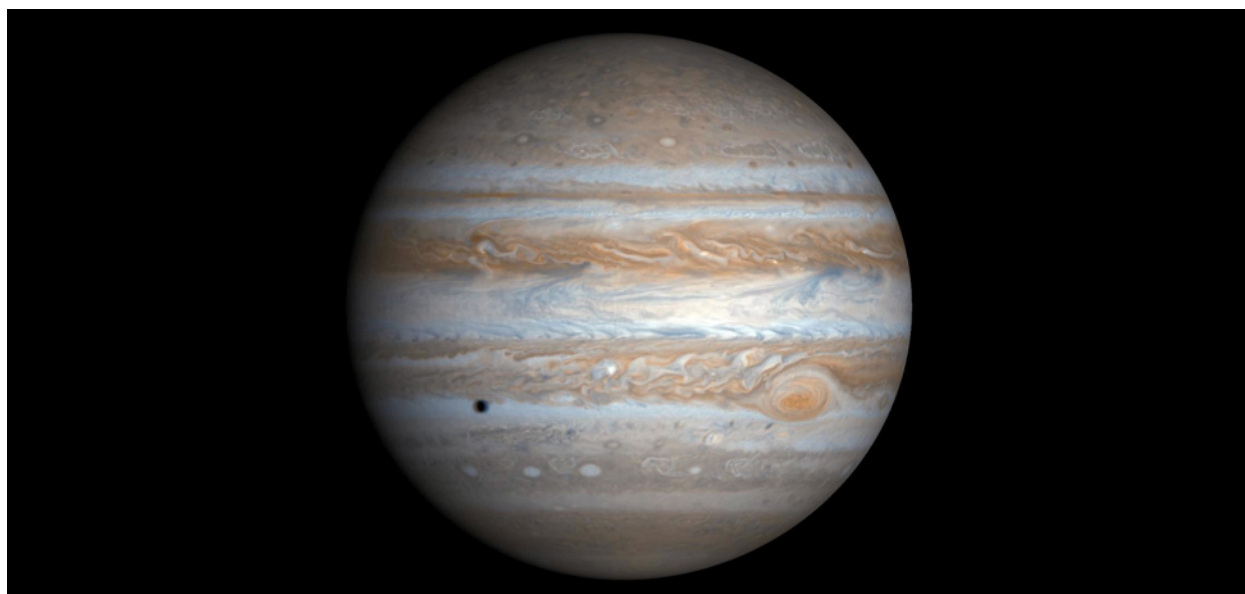
Figure 11.2. Jupiter. The Cassini spacecraft imaged Jupiter on its way to Saturn in 2012. The giant storm system called the Great Red Spot is visible to the lower right. The dark spot to the lower left is the shadow of Jupiter’s moon Europa. (credit: modification of work by NASA/JPL)
