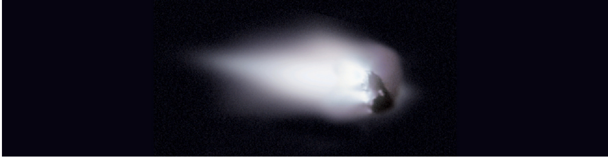
Figure 13.20. Close-up of Comet Halley. This historic photograph of the black, irregularly shaped nucleus of Comet Halley was obtained by the ESA Giotto spacecraft from a distance of about 1000 kilometers. The bright areas are jets of material escaping from the surface. The length of the nucleus is 10 kilometers, and details as small as 1 kilometer can be made out. (credit: modification of work by ESA)
