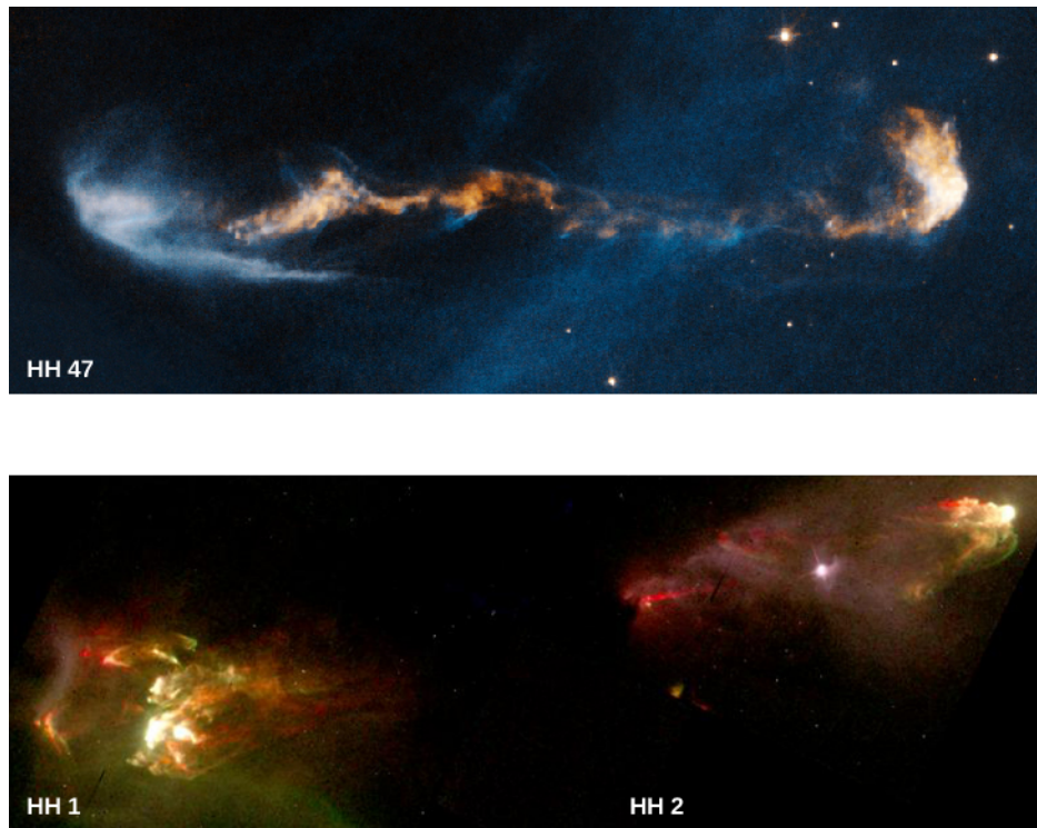
Figure 21.10. Outflows from Protostars. These images were taken with the Hubble Space Telescope and show jets flowing outward from newly formed stars. In the HH47 image, a protostar 1500 light-years away (invisible inside a dust disk at the left edge of the image) produces a very complicated jet. The star may actually be wobbling, perhaps because it has a companion. Light from the star illuminates the white region at the left because light can emerge perpendicular to the disk (just as the jet does). At right, the jet is plowing into existing clumps of interstellar gas, producing a shock wave that resembles an arrowhead. The HH1/2 image shows a double-beam jet emanating from a protostar (hidden in a dust disk in the center) in the constellation of Orion. Tip to tip, these jets are more than 1 light-year long. The bright regions (first identified by Herbig and Haro) are places where the jet is slamming into a clump of interstellar gas and causing it to glow. (credit “HH 47”: modification of work by NASA, ESA, and P. Hartigan (Rice University); credit “HH 1 and HH 2: modification of work by J. Hester, WFPC2 Team, NASA)
