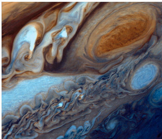
Figure 11.19. Jupiter's Great Red Spot. This is the largest storm system on Jupiter, as seen during the Voyager spacecraft flyby. Below and to the right of the Red Spot is one of the white ovals, which are similar but smaller high-pressure features. The white oval is roughly the size of planet Earth, to give you a sense of the huge scale of the weather patterns we are seeing. The colors on the Jupiter image have been somewhat exaggerated here so astronomers (and astronomy students) can study their differences more effectively. See Figure 11.2 to get a better sense of the colors your eye would actually see near Jupiter. (credit: NASA/JPL)
