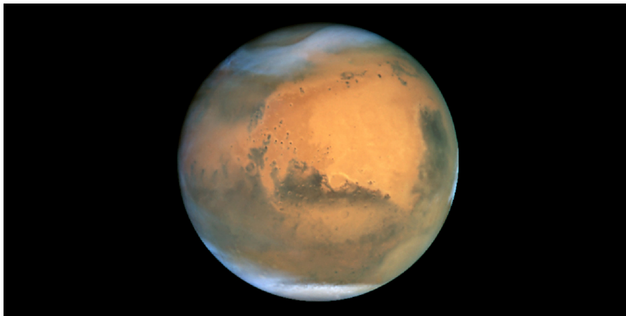
Figure 10.13. Mars Photographed by the Hubble Space Telescope. This is one of the best photos of Mars taken from our planet, obtained in June 2001 when Mars was only 68 million kilometers away. The resolution is about 20 kilometers—much better than can be obtained with ground-based telescopes but still insufficient to reveal the underlying geology of Mars. (credit: modification of work by NASA and the Hubble Heritage Team (STScI/AURA))
