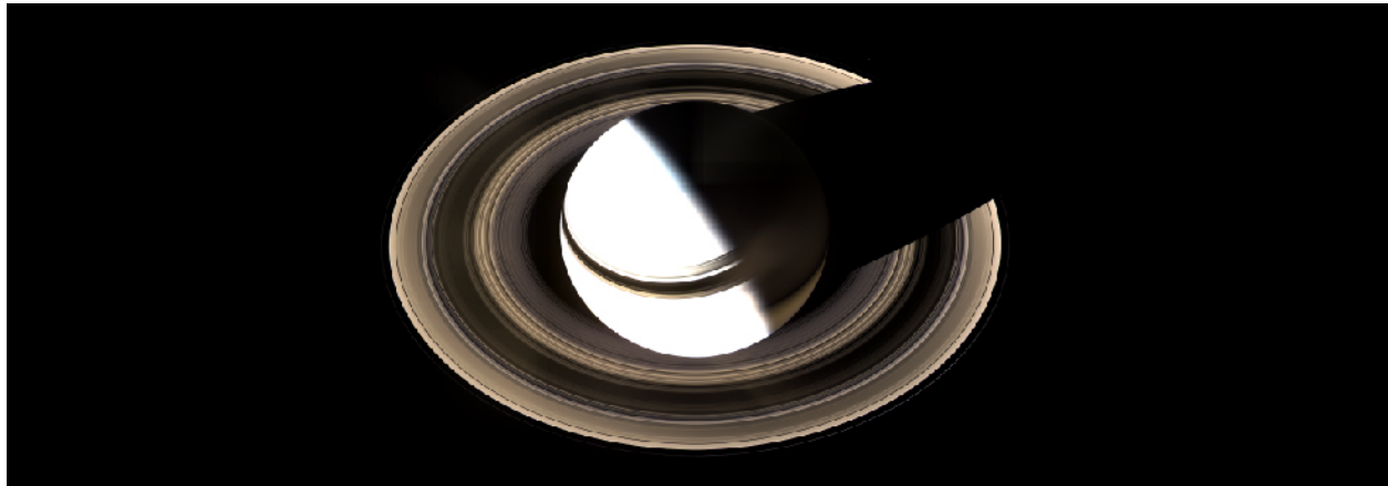
Figure 7.7. Saturn and Its Rings. This 2007 Cassini image shows Saturn and its complex system of rings, taken from a distance of about 1.2 million kilometers. This natural-color image is a composite of 36 images taken over the course of 2.5 hours. (credit: modification of work by NASA/JPL/Space Science Institute)
