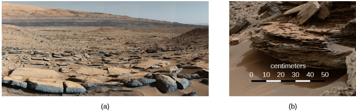
Figure 10.30. Gale Crater. (a) This scene, photographed by the Curiosity rover, shows an ancient lakebed of cracked mudstones. (b) Geologists working with the Curiosity rover interpret this image of cross-bedded sandstone in Gale crater as evidence of liquid water passing over a loose bed of sediment at the time this rock formed. (credit a: modification of work by NASA/JPL-Caltech/MSSS; credit b: modification of work by NASA/JPL-Caltech/MSSS)
