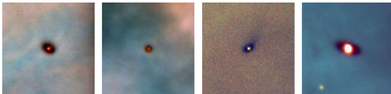
Figure 21.13. Disks around Protostars. These Hubble Space Telescope images show four disks around young stars in the Orion Nebula. The dark, dusty disks are seen silhouetted against the bright backdrop of the glowing gas in the nebula. The size of each image is about 30 times the diameter of our planetary system; this means the disks we see here range in size from two to eight times the orbit of Pluto. The red glow at the center of each disk is a young star, no more than a million years old. These images correspond to the stage in the life of a protostar shown in part (d) of Figure 21.8 . (credit: modification of work by Mark McCaughrean (Max-Planck-Institute for Astronomy), C. Robert O'Dell (Rice University), and NASA)
