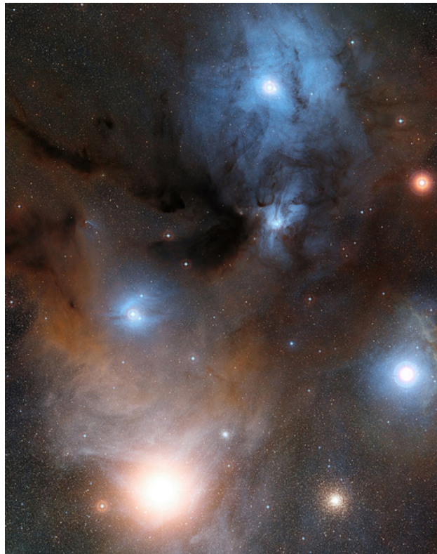
Figure 20.2. Various Types of Interstellar Matter. The reddish nebulae in this spectacular photograph glow with light emitted by hydrogen atoms. The darkest areas are clouds of dust that block the light from stars behind them. The upper part of the picture is filled with the bluish glow of light reflected from hot stars embedded in the outskirts of a huge, cool cloud of dust and gas. The cool supergiant star Antares can be seen as a big, reddish patch in the lower-left part of the picture. The star is shedding some of its outer atmosphere and is surrounded by a cloud of its own making that reflects the red light of the star. The red nebula in the middle right partially surrounds the star Sigma Scorpii. (To the right of Antares, you can see M4, a much more distant cluster of extremely old stars.) (credit: modification of work by ESO/Digitized Sky Survey 2)
