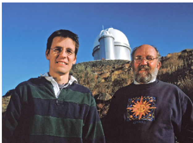
Figure 21.17. Planet Discoverers. In 1995, Didier Queloz and Michel Mayor of the Geneva Observatory were the first to discover a planet around a regular star (51 Pegasi). They are seen here at an observatory in Chile where they are continuing their planet hunting. (credit: Weinstein/Ciel et Espace Photos)
