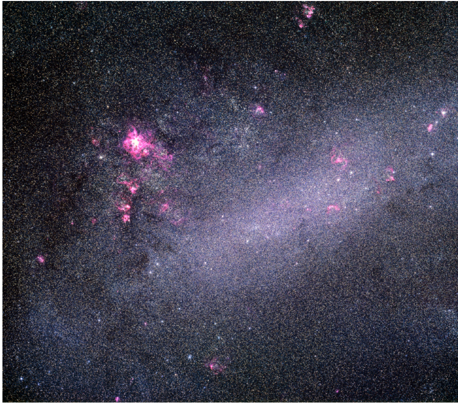
Figure 19.11. Large Magellanic Cloud. The Large Magellanic Cloud (so named because Magellan's crew were the first Europeans to record it) is a small, irregularly shaped galaxy near our own Milky Way. It was in this galaxy that Henrietta Leavitt discovered the cepheid period-luminosity relation. (credit: ESO)
