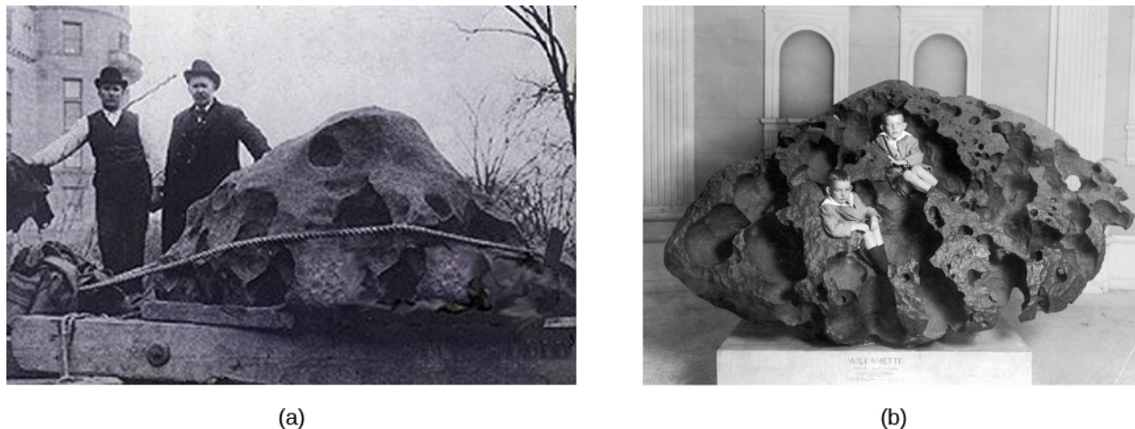
Figure 14.6. Meteorite Find. (a) This early twentieth century photo shows a 15-ton iron meteorite found in the Willamette Valley in Oregon. Although known to Native Americans in the area, it was “discovered” by an enterprising local farmer in 1902, who proceeded to steal it and put it on display. (b) It was eventually purchased for the American Museum of Natural History and is now on display in the museum’s Rose Center in New York City as the largest iron meteorite in the United States. In this 1911 photo, two young boys are perched in the meteor’s crevices.
