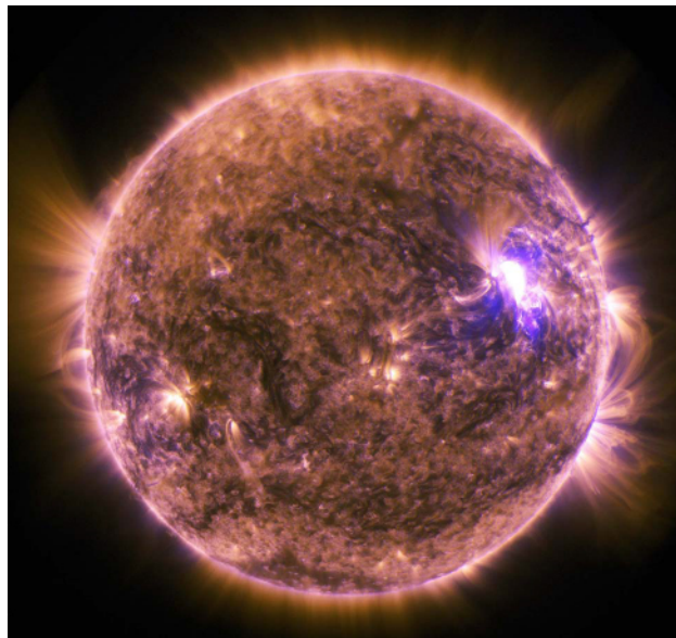
Figure 15.20. Solar Flare. The bright white area seen on the right side of the Sun in this image from the Solar Dynamics Observer spacecraft is a solar flare that was observed on June 25, 2015. (credit: NASA/SDO)
