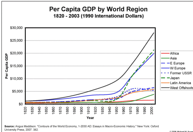
Figure 1: Evolution of global carbon emissions (top), world population (center) and per person GDP (bottom). From cdiac.ess-dive.lbl.gov , wikipedia.org , and krusekronicle.ty.pepad.com .
