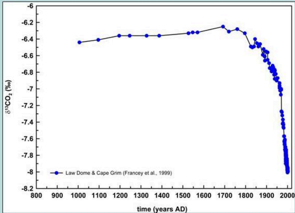
Reconstruction of the carbon isotope (C-13) of atmospheric CO 2 from the Law Dome ice core (Francey et al., 1999) and the Cape Grim ambient air measurements (Allison et al., 2003).
