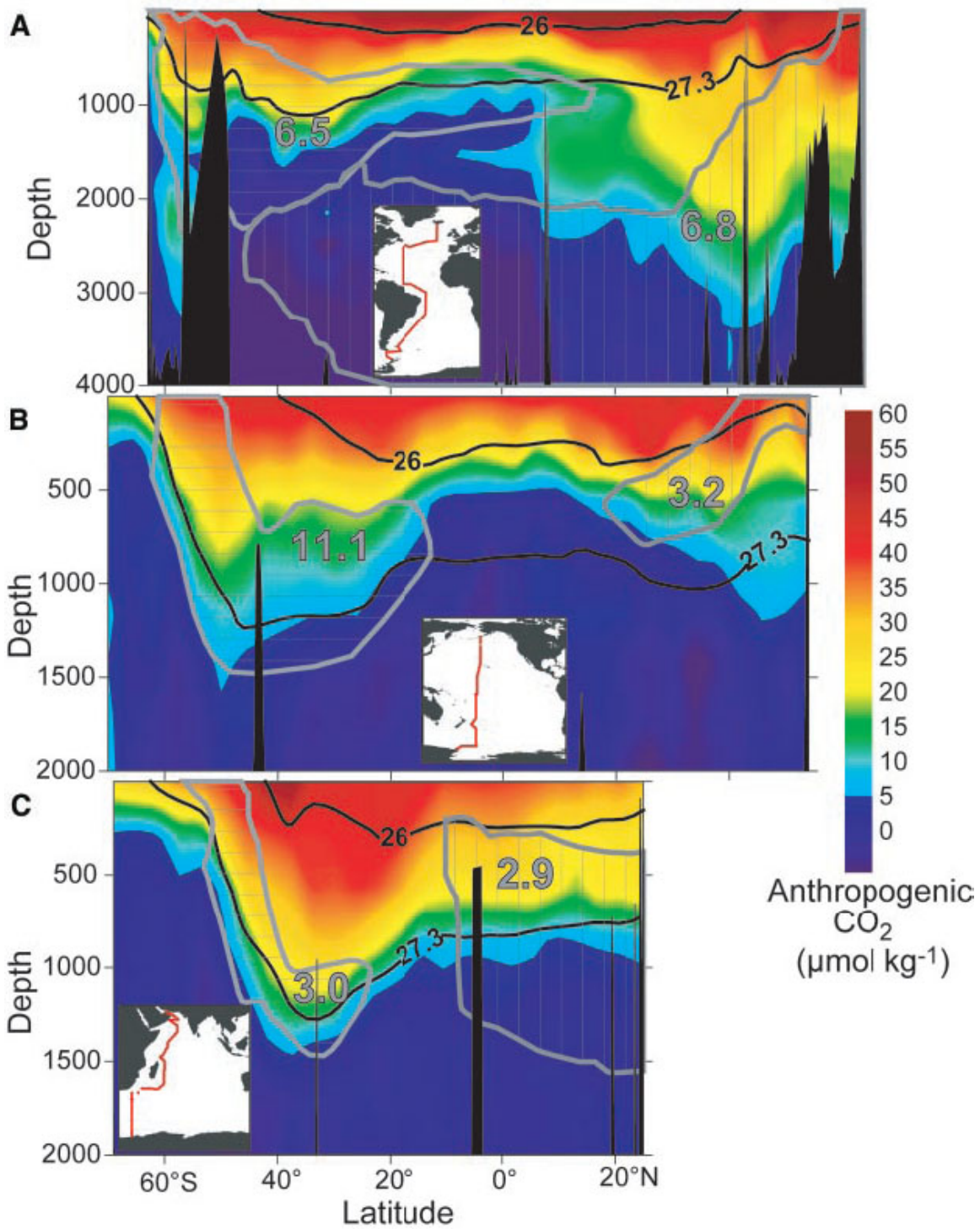
Figure 13: Latitude-depth sections of anthropogenic carbon in the Atlantic (A), Pacific (B), and Indian (C) oceans. Note that the depth scale is different in panel (A) from the other panels. Black lines denote two surfaces of constant potential density (expressed in \sigma_\theta = \text{density} - 1000 \text{ kg m}^{-3} ). Movements in the ocean are preferentially along lines of constant potential density because it requires no change in energy (adiabatic). Grey outlines and numbers denote different intermediate and deep water masses and their anthropogenic carbon content in PgC. From pmel.noaa.gov .
