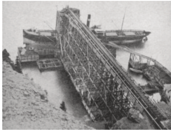
Figure 3.3 Iron ore from Bell Island is loaded onto a metal-hulled ship, ca. 1903.
