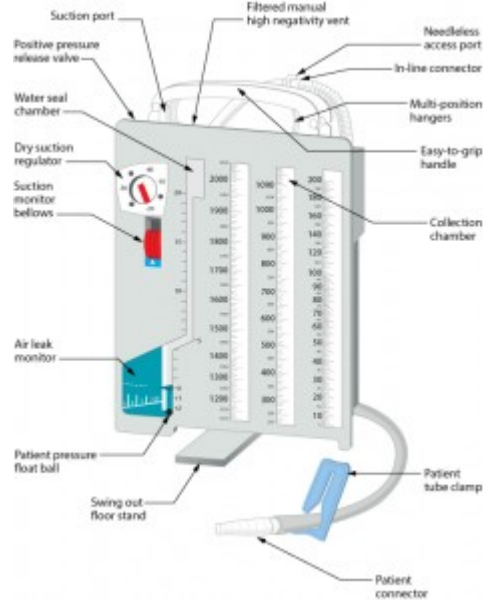
Figure 10.6 Chest tube drainage system with labelled parts
