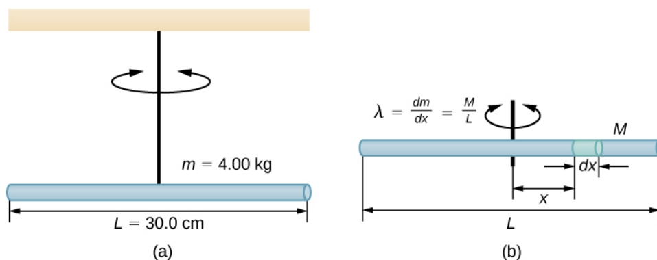
Figure 15.23 (a) A rod suspended by a string from the ceiling. (b) Finding the rod's moment of inertia.
