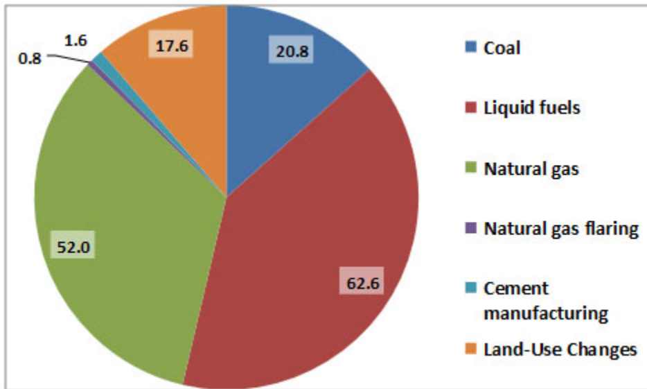
Figure 17.4. Major Sources of CO 2 Emissions to the Atmosphere in Canada. Data are for 2004 and are in 10^6 tC/y. Data for coal, petroleum, and natural gas are related to combustion sources, while land-use changes are mostly disturbances of natural ecosystems. Source: Data from CDIAC (2015)
