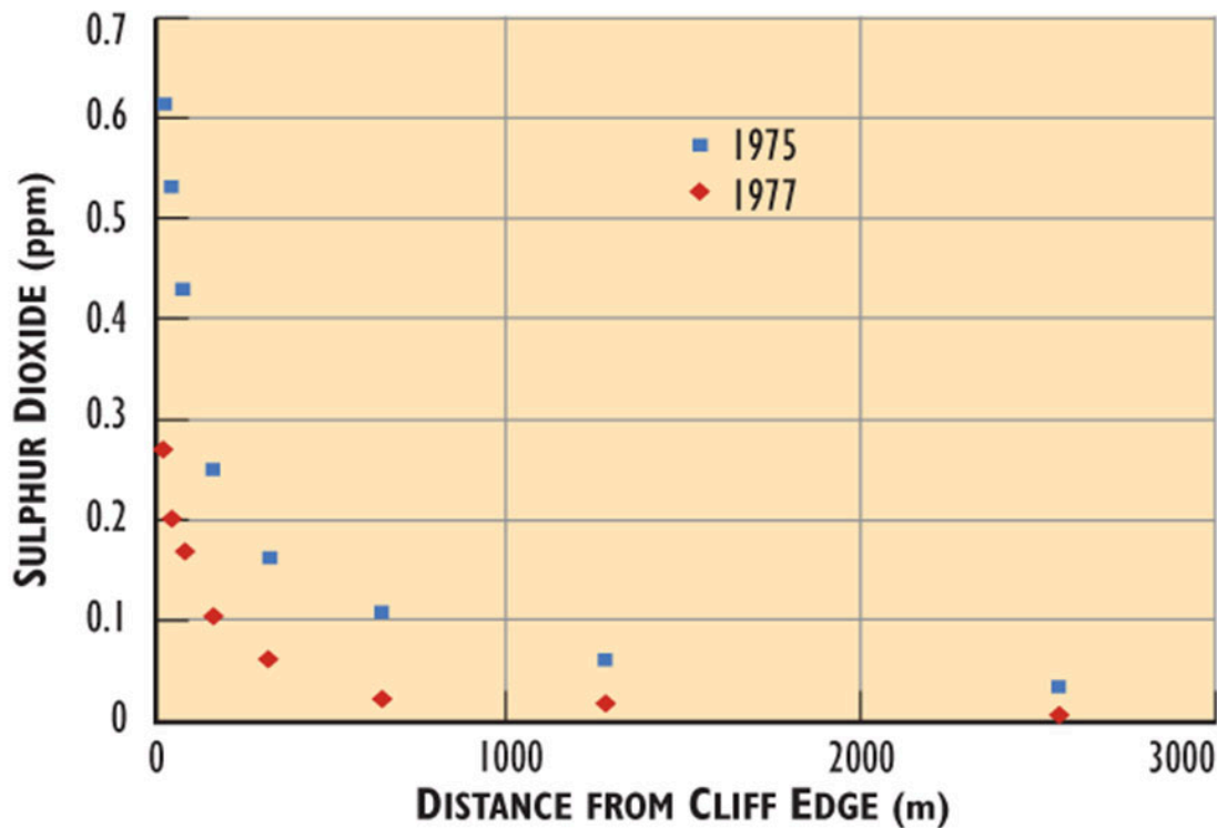
Figure 16.5. Sulphur Dioxide at the Smoking Hills. The data are averages of 8- and 14-day sampling periods, respectively. The averages include times when SO 2 concentrations were high, as well as those when the sampling sites were not fumigated because the plumes were blowing out to sea. Source: Data from Gizyn (1980).
