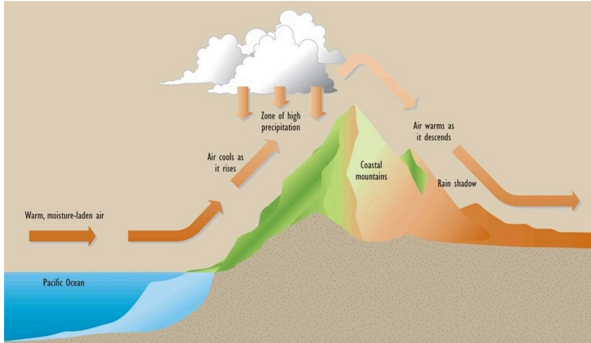
Figure 3.3. A diagrammatic model of orographic precipitation.
