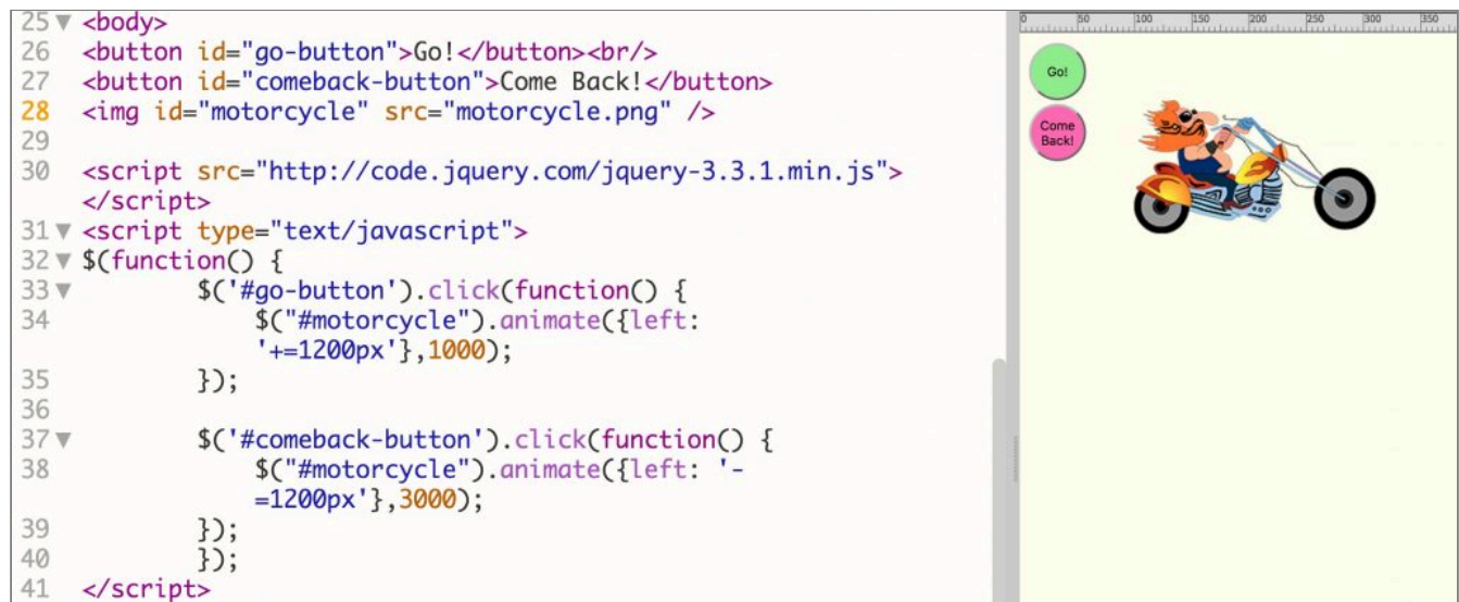
Figure 8-4. Simple animation done with jQuery, which allows for user interaction via the two buttons. dobe® Dreamweaver® screenshot(s) reprinted with permission from Adobe Systems Incorporated.
