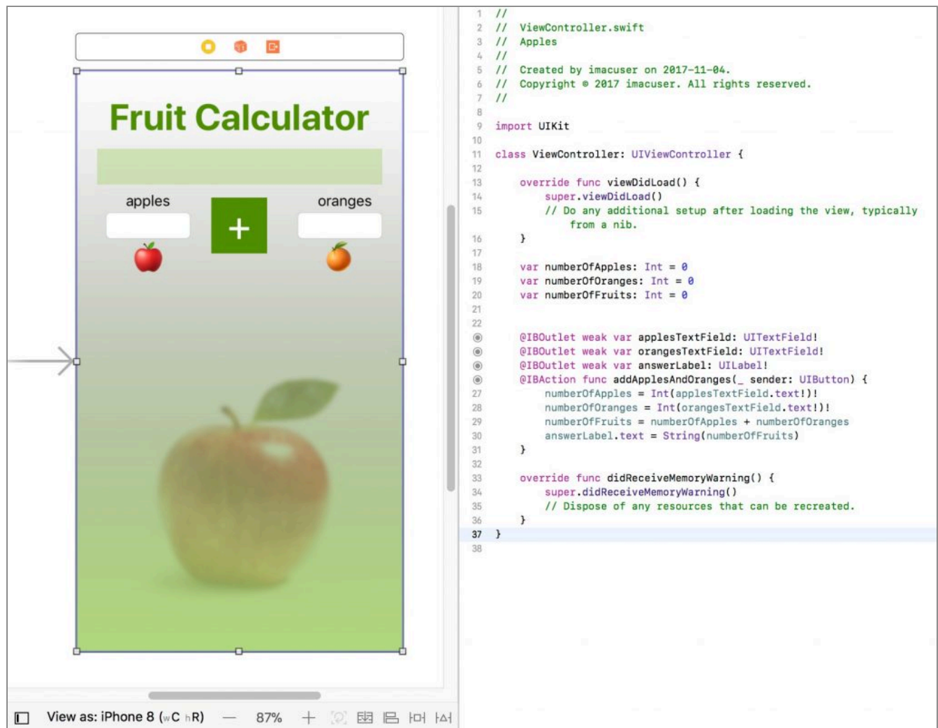
Figure 16-1a. Interface of Apple Xcode, the MacOS program for writing apps for the iPhone and iPad. The Storyboard with screen layout is shown at left and the ViewController with code at right. Screen shot(s) reprinted with permission from Apple Inc.
