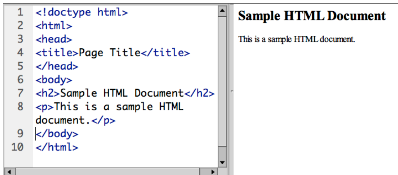
Figure 1-1. Structure of a basic HTML page for viewing with a web browser. Adobe® Dreamweaver® screenshot(s) reprinted with permission from Adobe Systems Incorporated.
