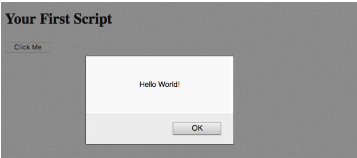
Figure 9-1. Javascript Alert
