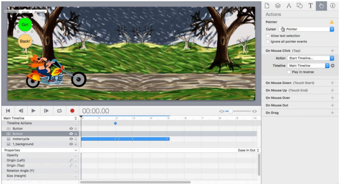
Figure 8-5. Screenshot of Tumult Hype animation showing the stage, timeline, keyframe properties, and inspector. Tumult Hype. Reprinted with permission.
