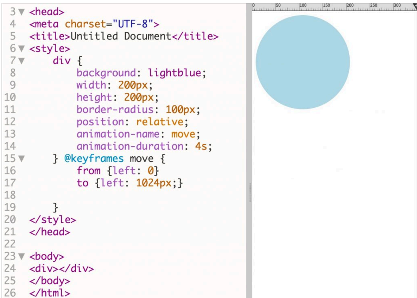
Figure 8-3. Example of the @keyframes rule (line 15) and animate style (lines 13 and 14) applied to a circular div. When the page is loaded, the div moves across the page from left to right. dobe® Dreamweaver® screenshot(s) reprinted with permission from Adobe Systems Incorporated.
