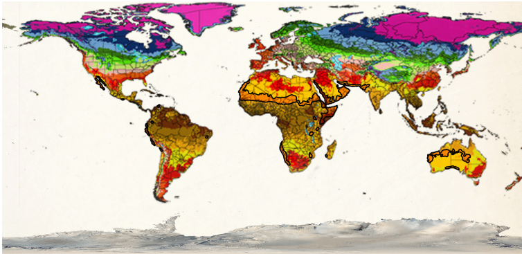
Figure 24: Koppen Geiger map with plant hardiness zones overlaid. Orange areas surrounded by black lines are areas of overlap between the Koppen Geiger classification and the plant hardiness zone.
