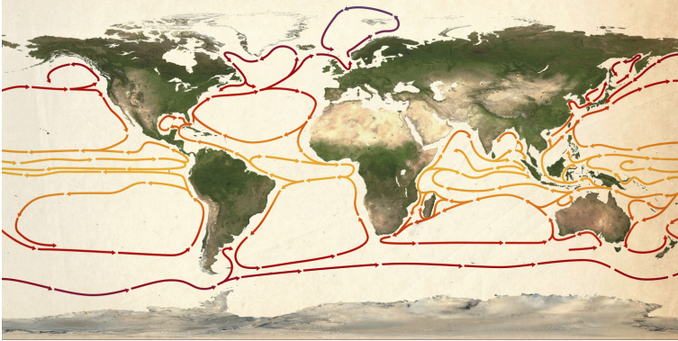
Figure 6: Ocean Currents
