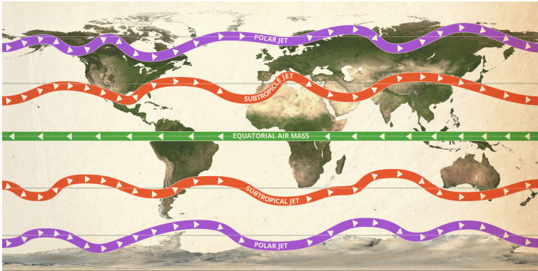
Figure 5: Jet Streams
