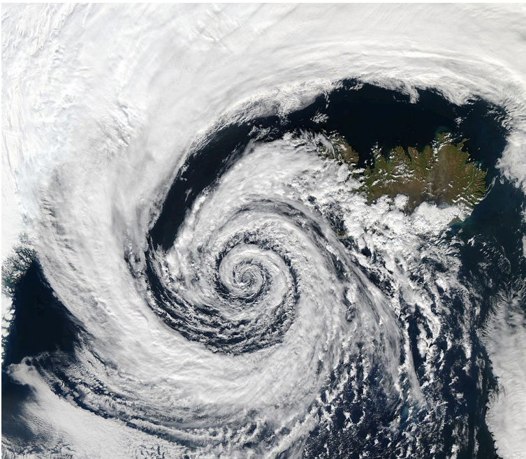
Figure 66: A Cyclone over Iceland. Image by NASA
