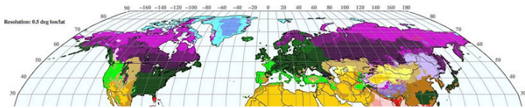
Projected Northern Hemisphere 2076-2100
