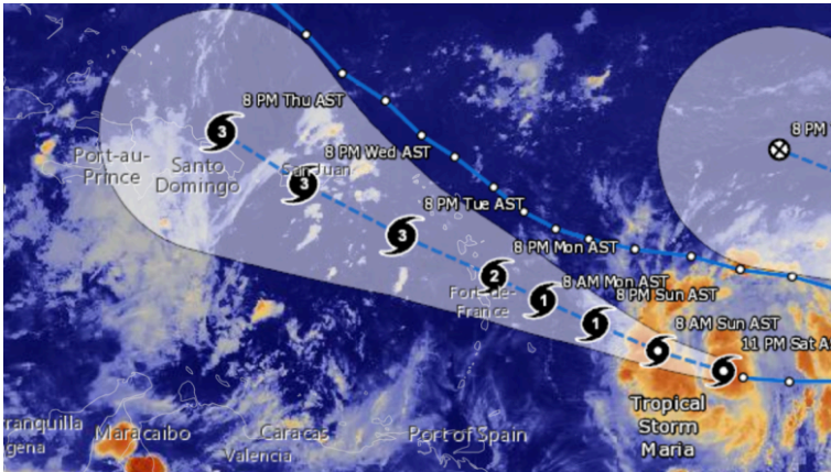
Figure 71: Hurricane Marie Forecast. Image by NOAA
