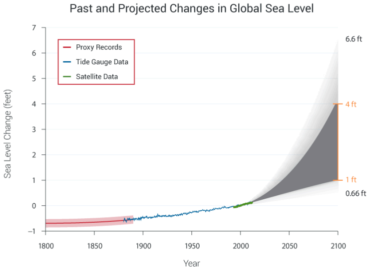
Figure 75: Past and Projected Changes in Global Sea Level Rise. By the National Climate Assessment
