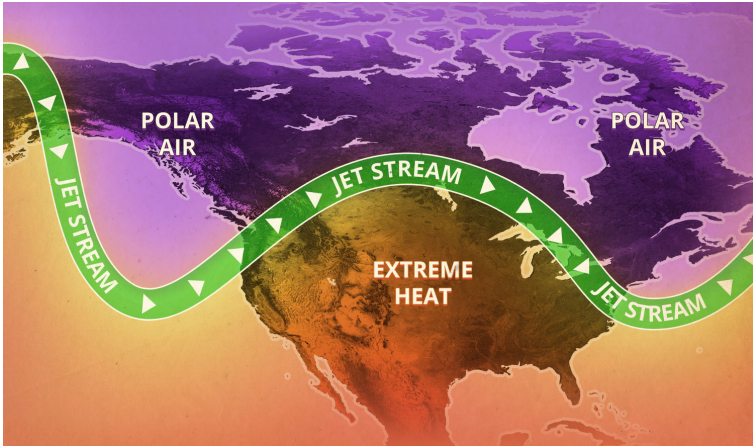
Figure 4: Heat Wave
