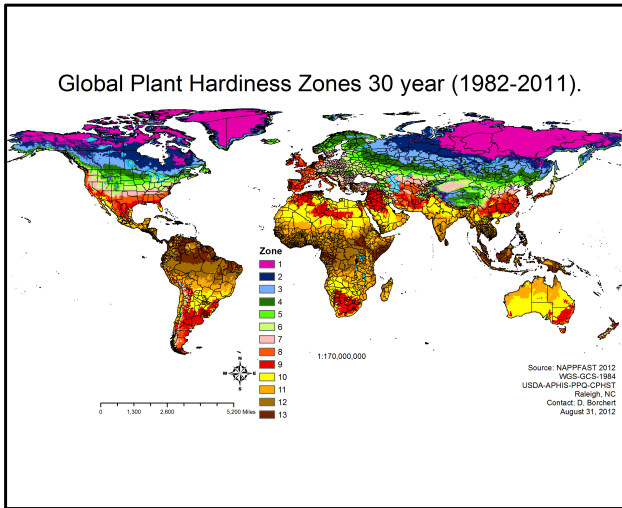
Figure 10: Global Plant Hardiness Zones 30 Year (1982-2011)
