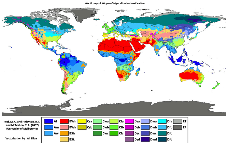
Figure 11: World map of Köppen-Geiger Climate Classification.
