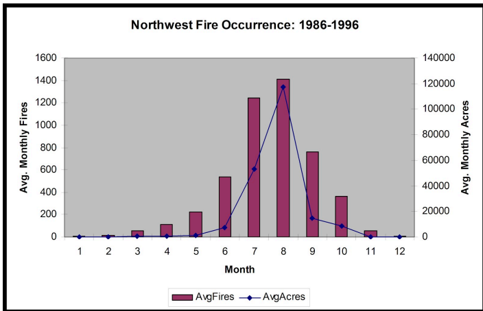
Figure 57: Northwest Fire Occurrence: 1986-1996
