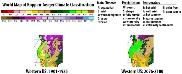
Figure 36: Corvallis on the Koppen Geiger Map 1901-1925 and 2076-2100
