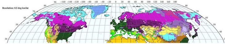
Northern Hemisphere 1901-1925
