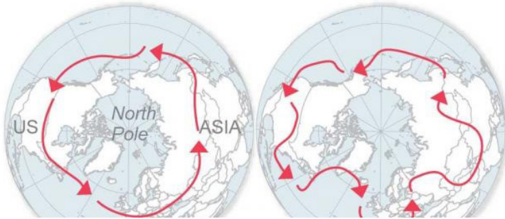
Figure 28: Path of Northern Jet Stream Changes
