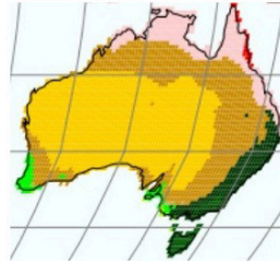
Projected Australia Koppen Geiger Map 2076-2100
