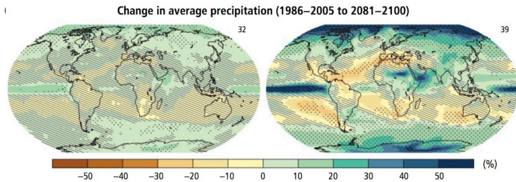
Figure 30: Change in Average Precipitation (1986-2005 to 2081-2100)
