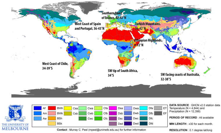
Figure 42: Climate analogues worth investigating.
