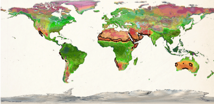
Figure 25: Koppen Geiger with plant hardiness zones overlaid with precipitation zones. Areas within the black line are overlapped between the Koppen Geiger zone, plant hardiness zone, and the annual precipitation.
