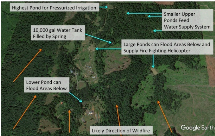
Figure 63: Cougar Mountain Sanctuary Water Storage
