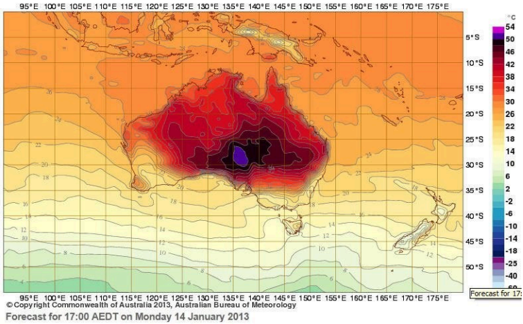
Figure 56: Australian Temperature Map
