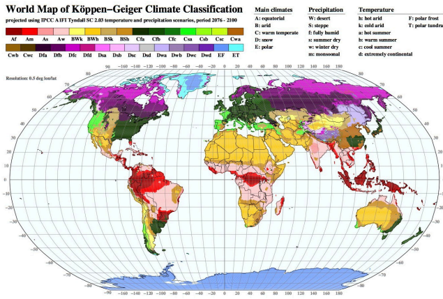
Figure 2: World Map of Köppen-Geiger climate classification projected with Tsydal temperature and precipitation data for the period 2076-2100, A1FI emission scenario, on a regular 0.5 degree latitude/longitude grid.
