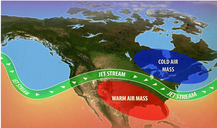
Figure 27: Jet Stream through the US.
