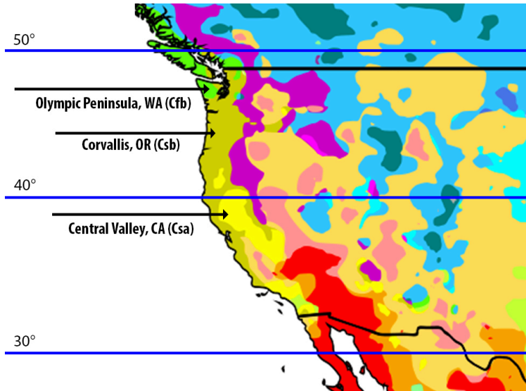
Figure 13: West Coast Climate Types
