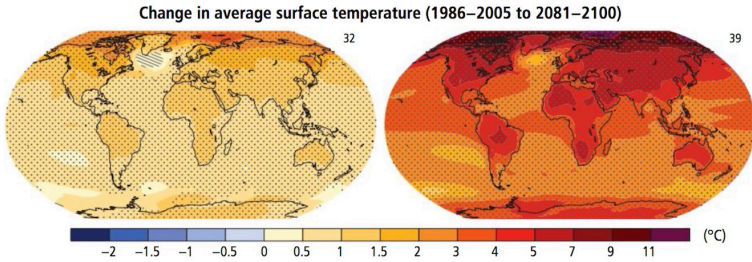
Figure 32: Change in Average Surface Temperature (1986–2005 to 2081–2100)
