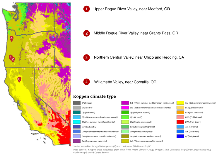
Figure 38: Köppen Climate Map with climate analogues pinpointed.
