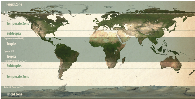
Figure 1: Climate Zones
