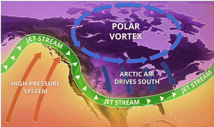
Figure 3: Polar Vortex
