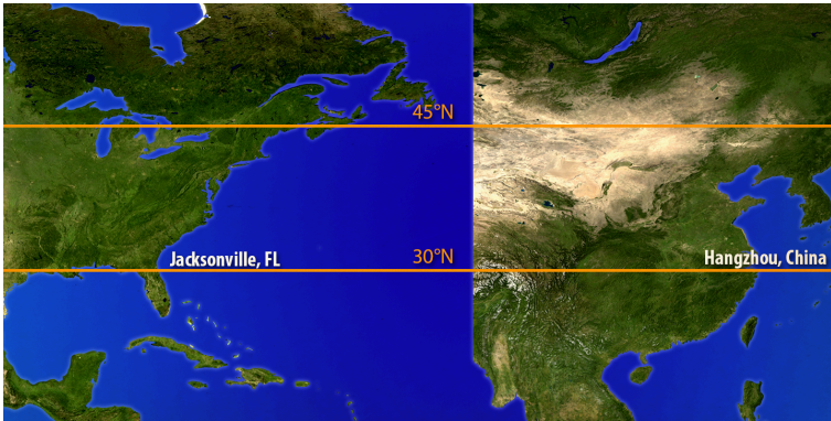
Figure 20: Climate Analogue for Jacksonville and Hangzhou, China
