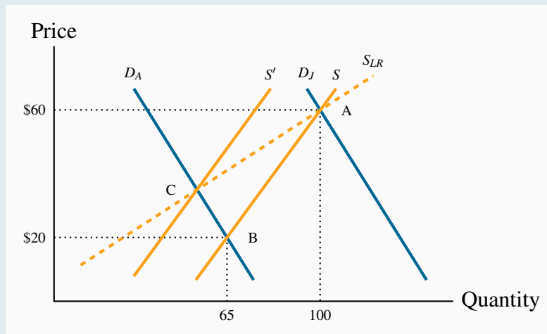
Figure 4.7: Supply elasticity in the short run and the long run; the oil market in 2020
