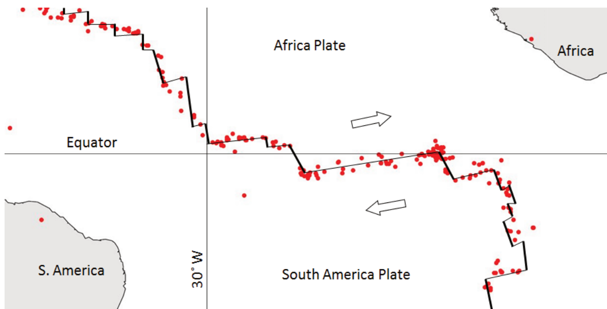
Figure 4.8.2 Earthquake activity along the mid Atlantic ridge (Steven Earle, “Physical Geology”).
