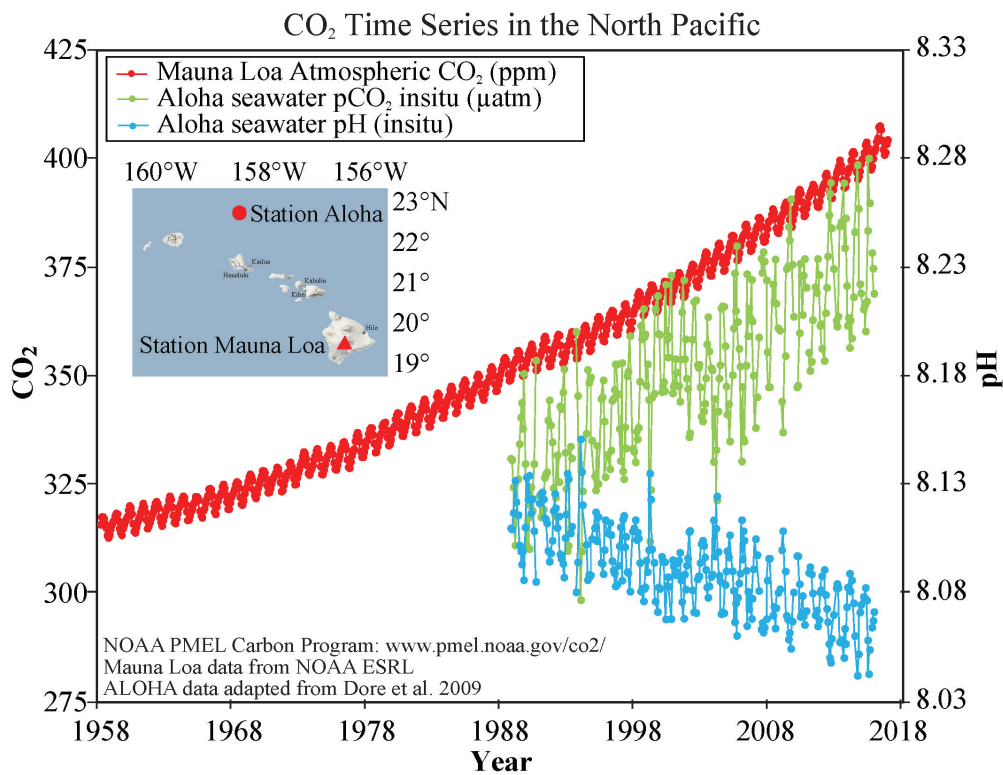
Figure 5.5.3 Changes in atmospheric CO 2 (red), seawater CO 2 (green) and pH (blue) in the Hawaiian Islands (NOAA PMEL).
