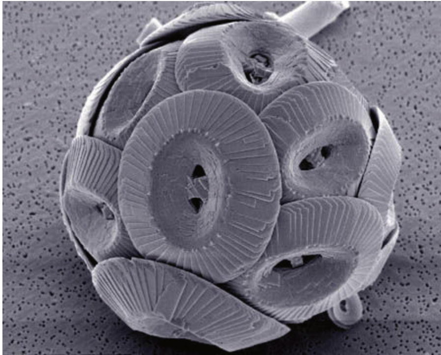
Figure 7.2.3 Electron microscope image of the North Atlantic coccolithophore Coccolithus pelagicus (Richard Lampitt, Jeremy Young, The Natural History Museum, London ( http://planktonnet.awi.de/ ) [CC BY 2.5], via Wikimedia Commons).
