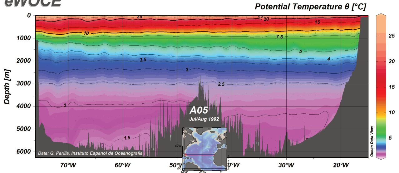
Figure 6.2.3 Temperature profile across the Atlantic Ocean from the coast of Florida to the coast of Africa (inset). There is rapid temperature change near the surface in the thermocline zone, but the deep water temperature is fairly stable (eWOCE, http://www.ewoce.org/gallery/eWOCE_Tables.html#Atlantic ).
