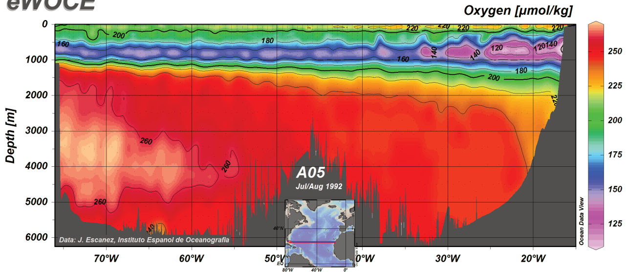
Figure 5.4.2 Dissolved oxygen profile from a transect across the Atlantic Ocean from Florida to the coast of Africa (inset). The oxygen minimum layer is visible between 500-1000 m (eWOCE, http://www.ewoce.org/gallery/eWOCE_Tables.html#Atlantic ).
