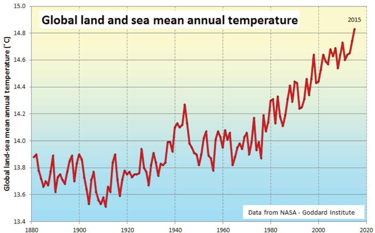
Figure 8.5.2 Global mean annual temperatures for the period from 1880 to 2015 (Steven Earle, "Physical Geology", by SE from data at NASA at: http://data.giss.nasa.gov/gistemp/tabledata_v3/GLB.Ts+dSST.txt ).
